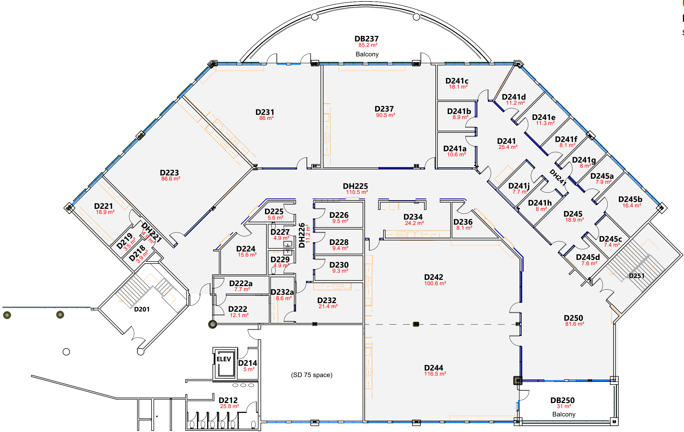
Upper Floor 1 : 200
